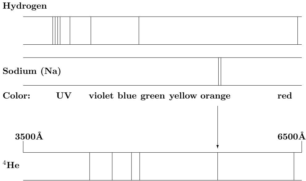
Figure 7. Absorption lines of hydrogen, sodium and 4 He (schematic). The absorption line of helium marked with an arrow (discovered in August and October 1868 [75]) is very close to the characteristic pair of absorption lines of sodium (Na) around 5890Å, but has a somewhat shorter wavelength. Three other absorption lines of helium are close to three absorption lines of hydrogen. Strong absorption lines of hydrogen and sodium may mask these absorption lines of helium in a blurry or faint spectra. The UV (Ultra Violet) 584.33Å, 537.03Å and 304Å absorption lines of helium are not shown here because they are too far to the left. Å denotes Angström = 10 -10 meter
