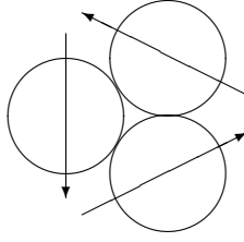
Figure 5. A baryon with zero total spin: In this configuration the resultant spin vector of the three half-spin quarks is zero [21]
