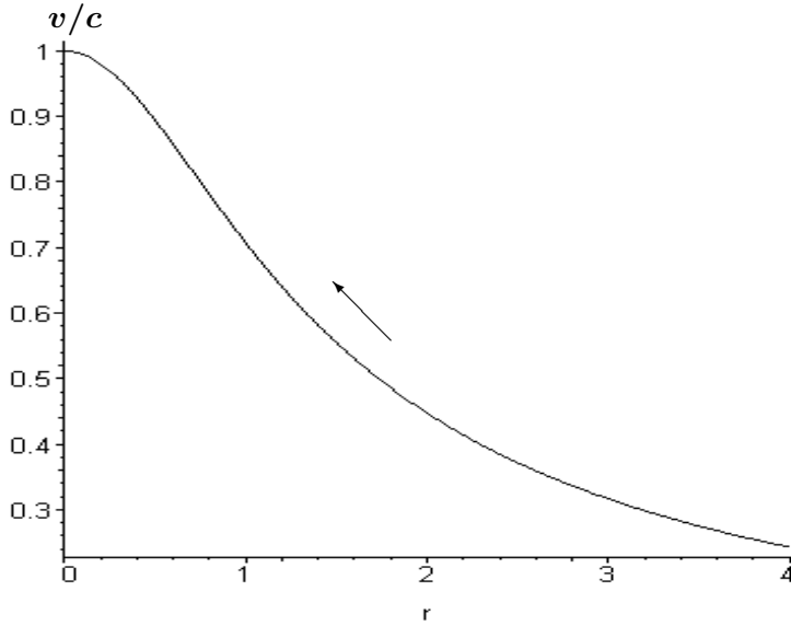
Figure 6. Circumferential velocity v(\mathbf{r}) (21) of two bodies orbiting each other and approaching towards a collision (schematic). The collision occurs when r = r_1 + r_2
